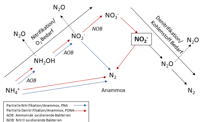
Fig. 1: N 2 O-Formation in wastewater treatment plants
