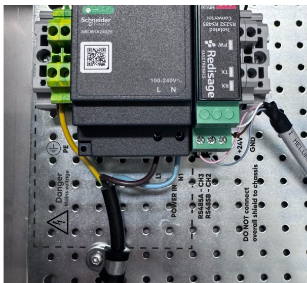
Picture 1A: Cables inside the N 2 O Wastewater Operator Console (Engraving visualization)
