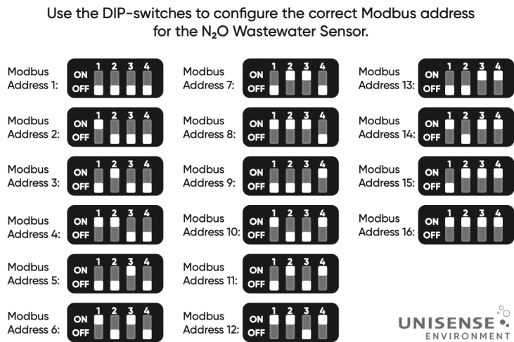
Figure 2: DIP-switch diagram
